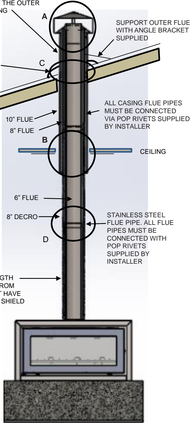
FRONT VIEW
